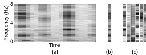
Figure 1: Comparison of noise models. (a) A spectrogram of 20 frames of computer keyboard noise. (b) Classical speech enhancement algorithms like spectral subtraction model noise with a single spectrum, e.g. the average spectrum. (c) Non-negative spectrogram decomposition uses a dictionary (multiple basis spectra). The latter is suitable for non-stationary noise.
